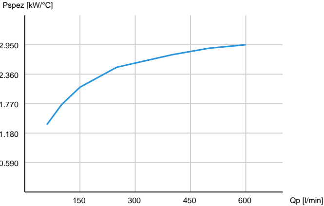
Cooling Performance*
